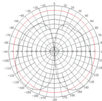
V polarization
